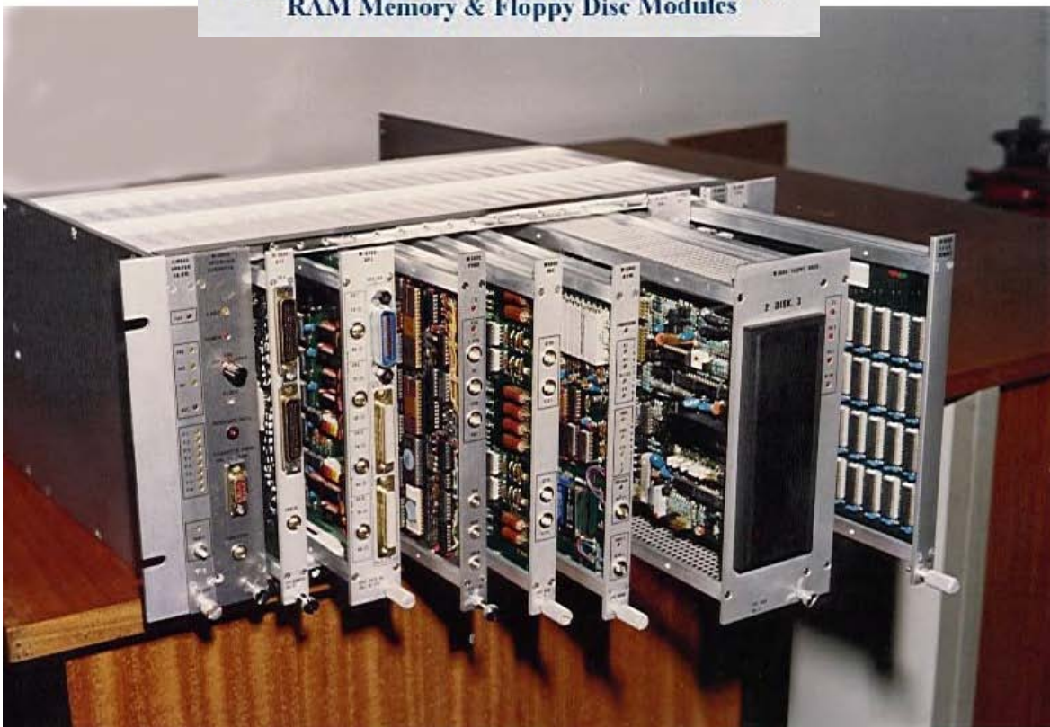
CIMBUS 19" Chassis & CPU, RS 232, IEEE 488, RAM Memory & Floppy Disc Modules
